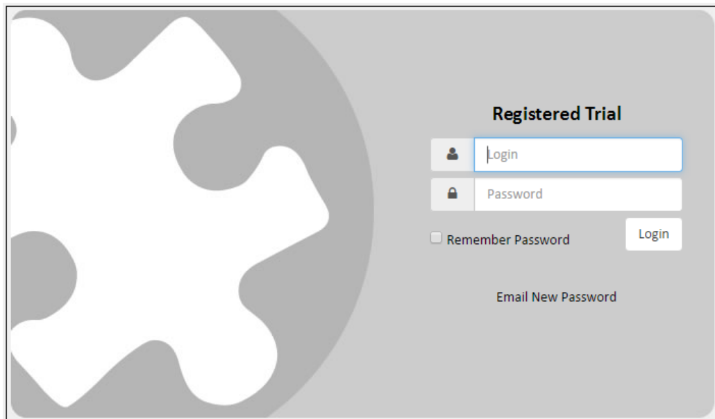
Figure 3: Login Screen
