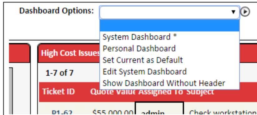
Figure 44: Dashboard Options
